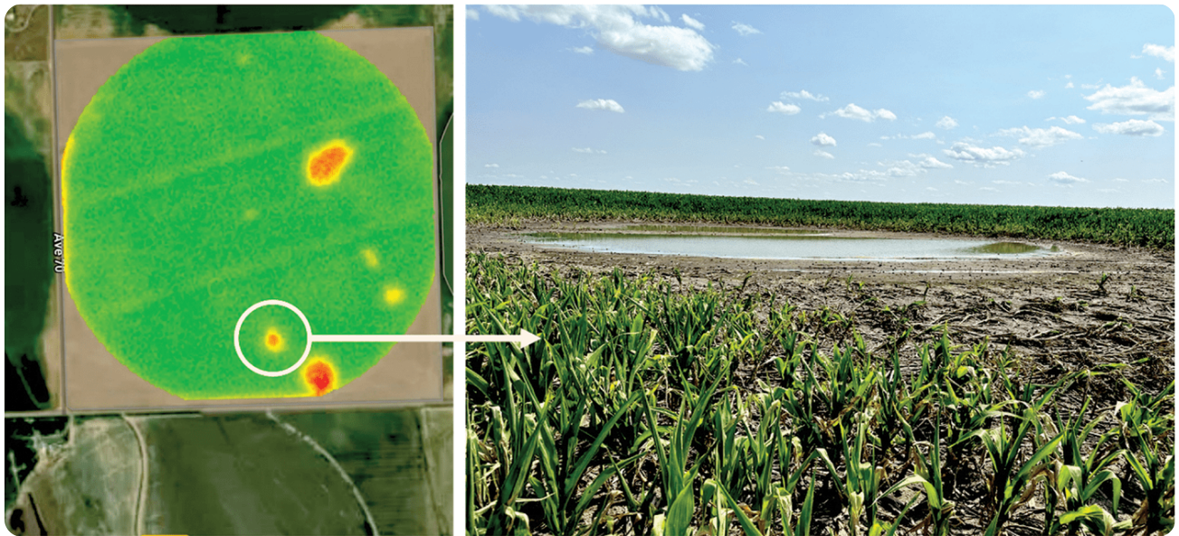
Left: Satellite imagery with a normalized difference red edge (NDRE) layer of a corn field in west-central Nebraska; Right: Photo taken of the actual site during field scouting.
